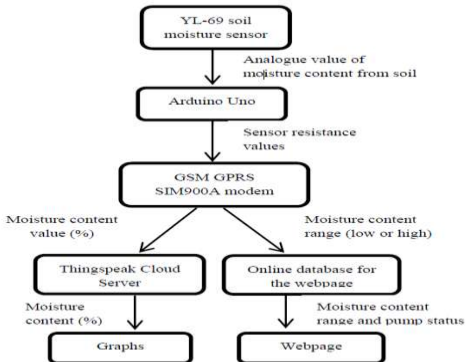
Figure 4 : Flow chart of the system
